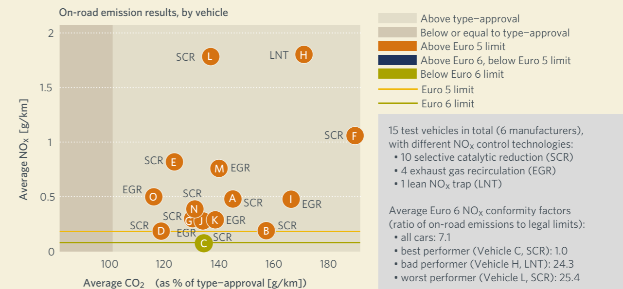
FIGURE 3 - ON-ROAD VEHICLE EMISSIONS, GROUPED BY AFTER-TREATMENT TECHNOLOGY. EURO 5 AND EURO 6 LIMITS ARE IDENTIFIED.
