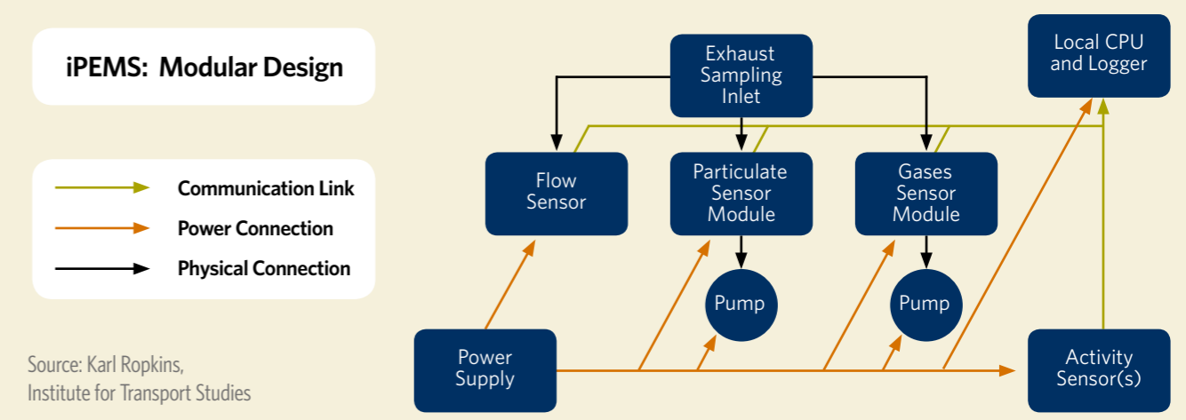
FIGURE 5: SCHEMATIC OF IPEMS DESIGN
